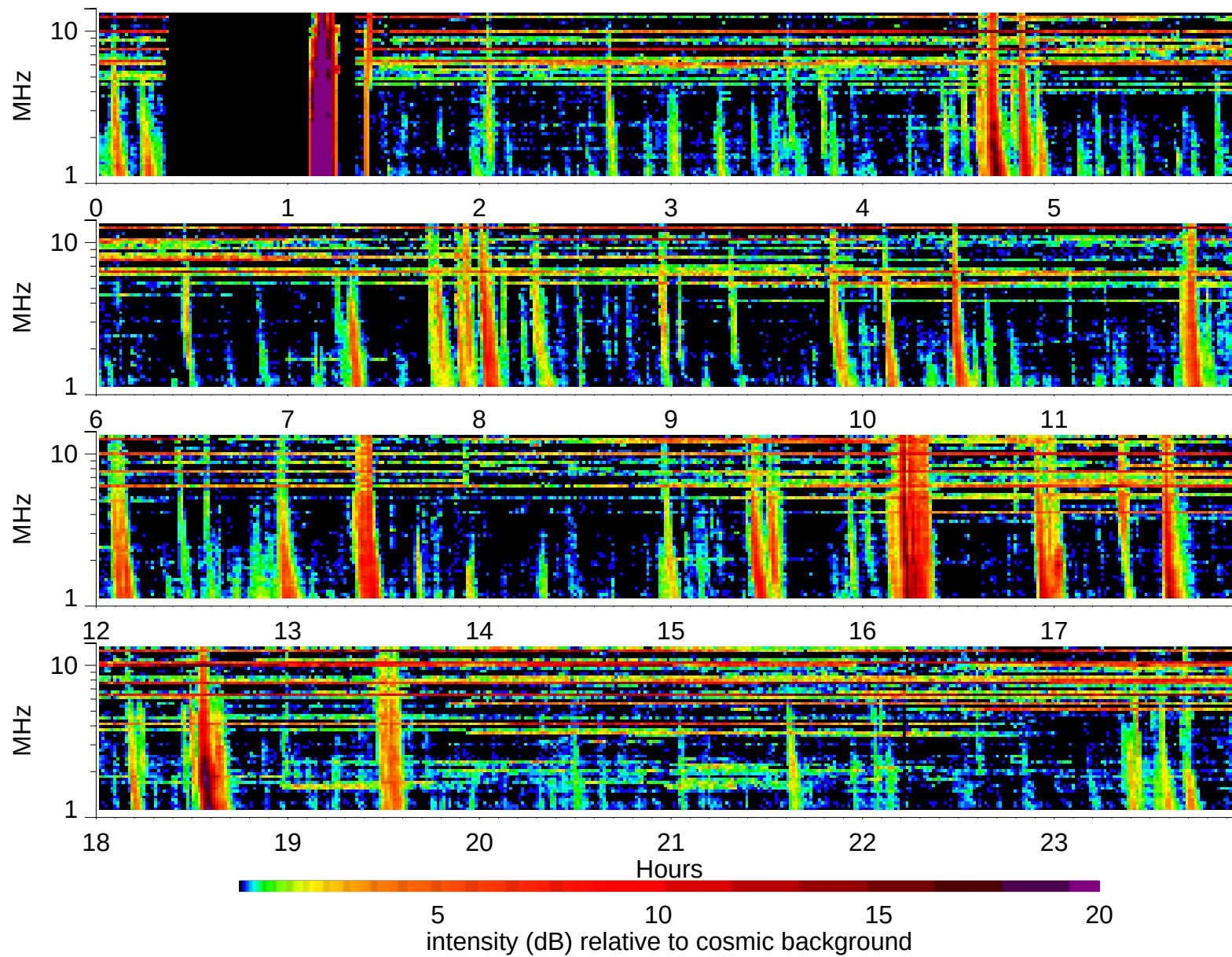
Wind Waves RAD2 receiver: 1999/12/26
