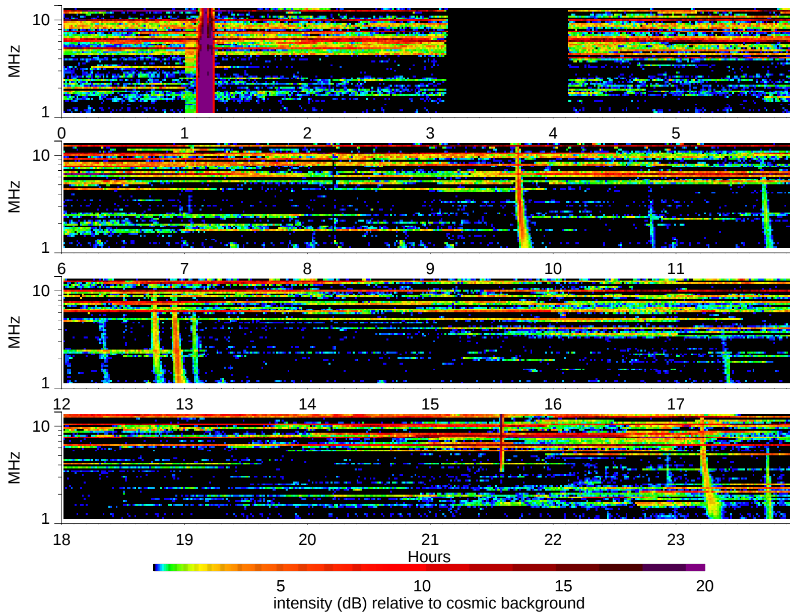
Wind Waves RAD2 receiver: 1999/12/30
