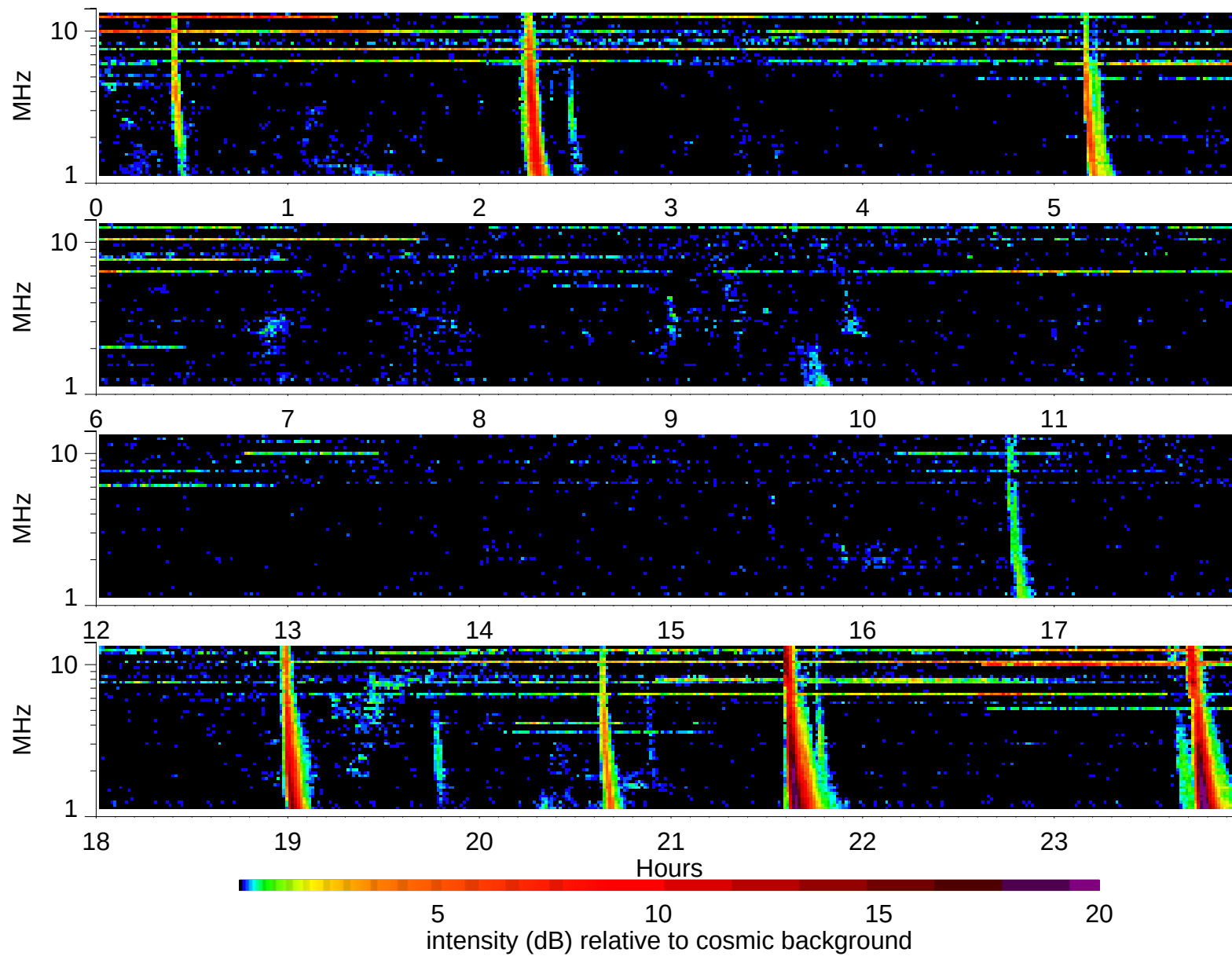
Wind Waves RAD2 receiver: 2002/1/3
