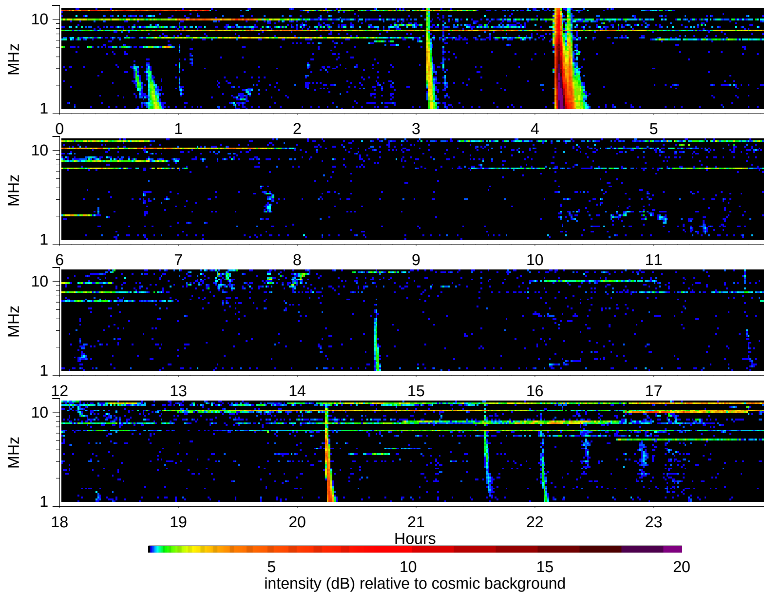
Wind Waves RAD2 receiver: 2002/1/5
