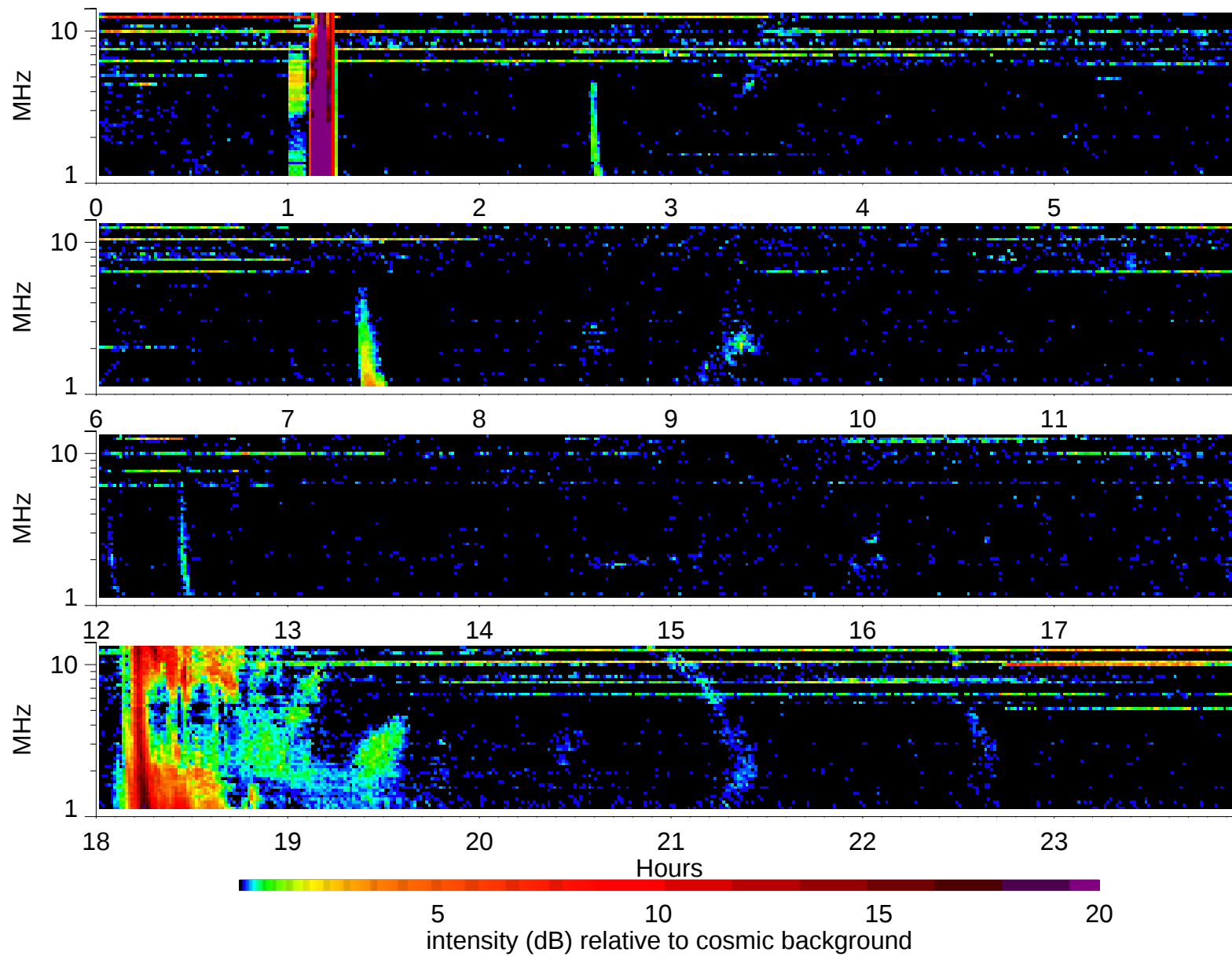
Wind Waves RAD2 receiver: 2002/1/8
