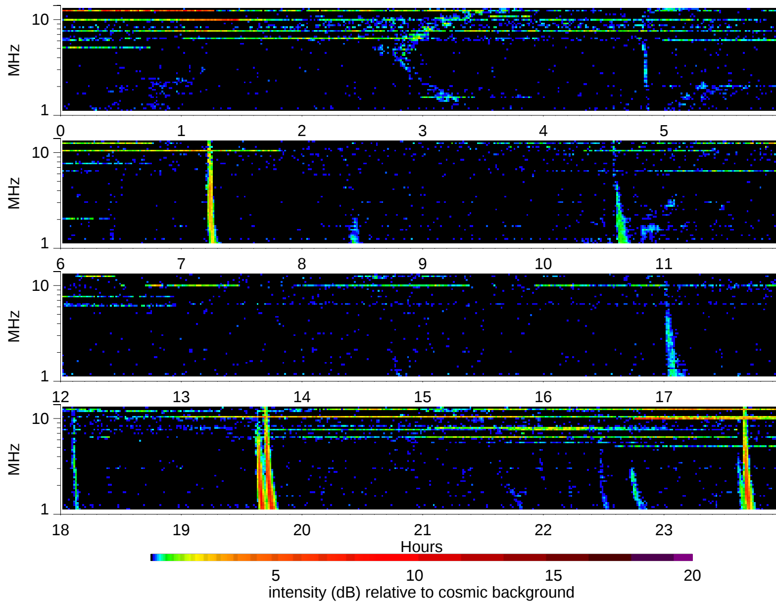
Wind Waves RAD2 receiver: 2002/1/9
