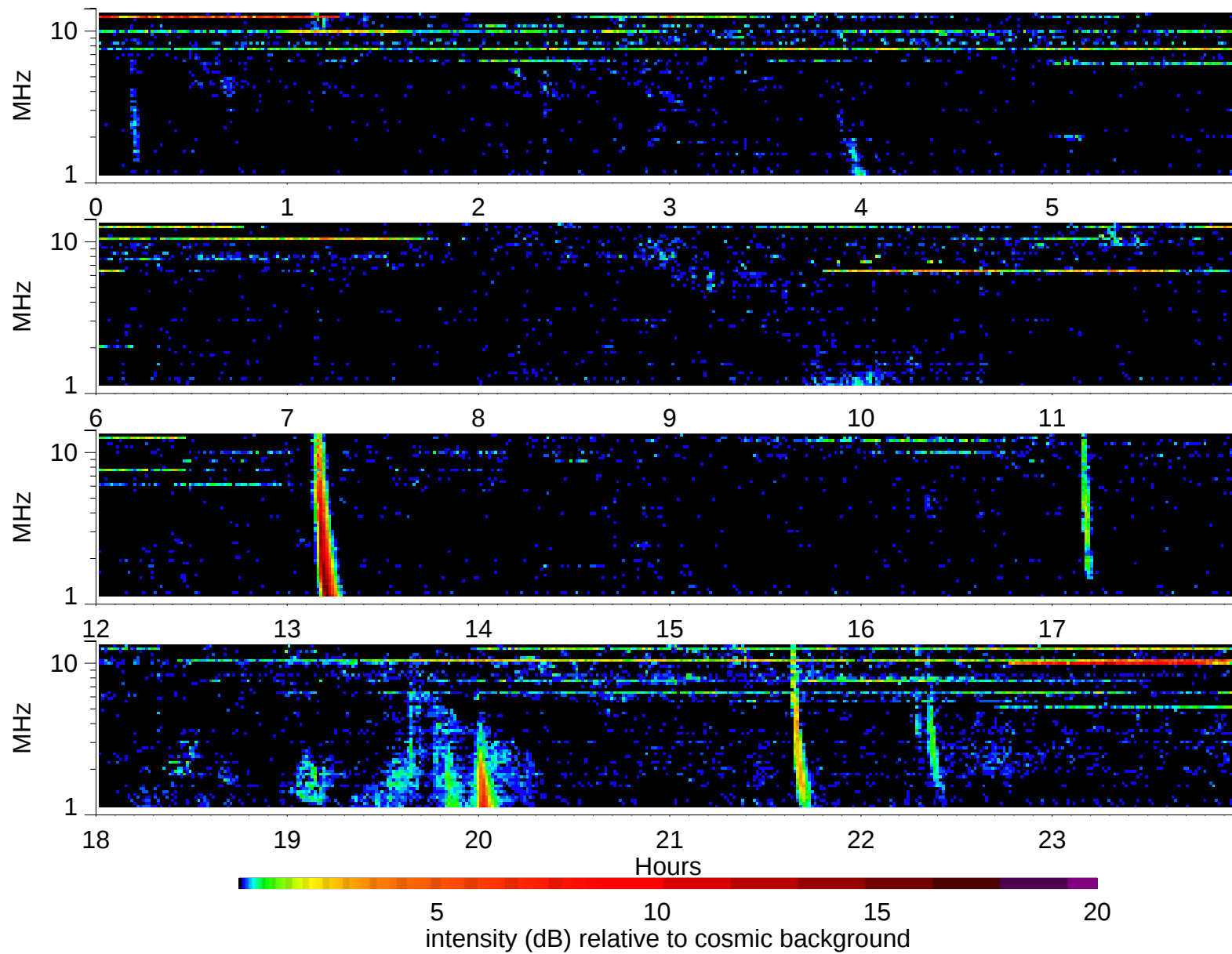
Wind Waves RAD2 receiver: 2002/1/13
