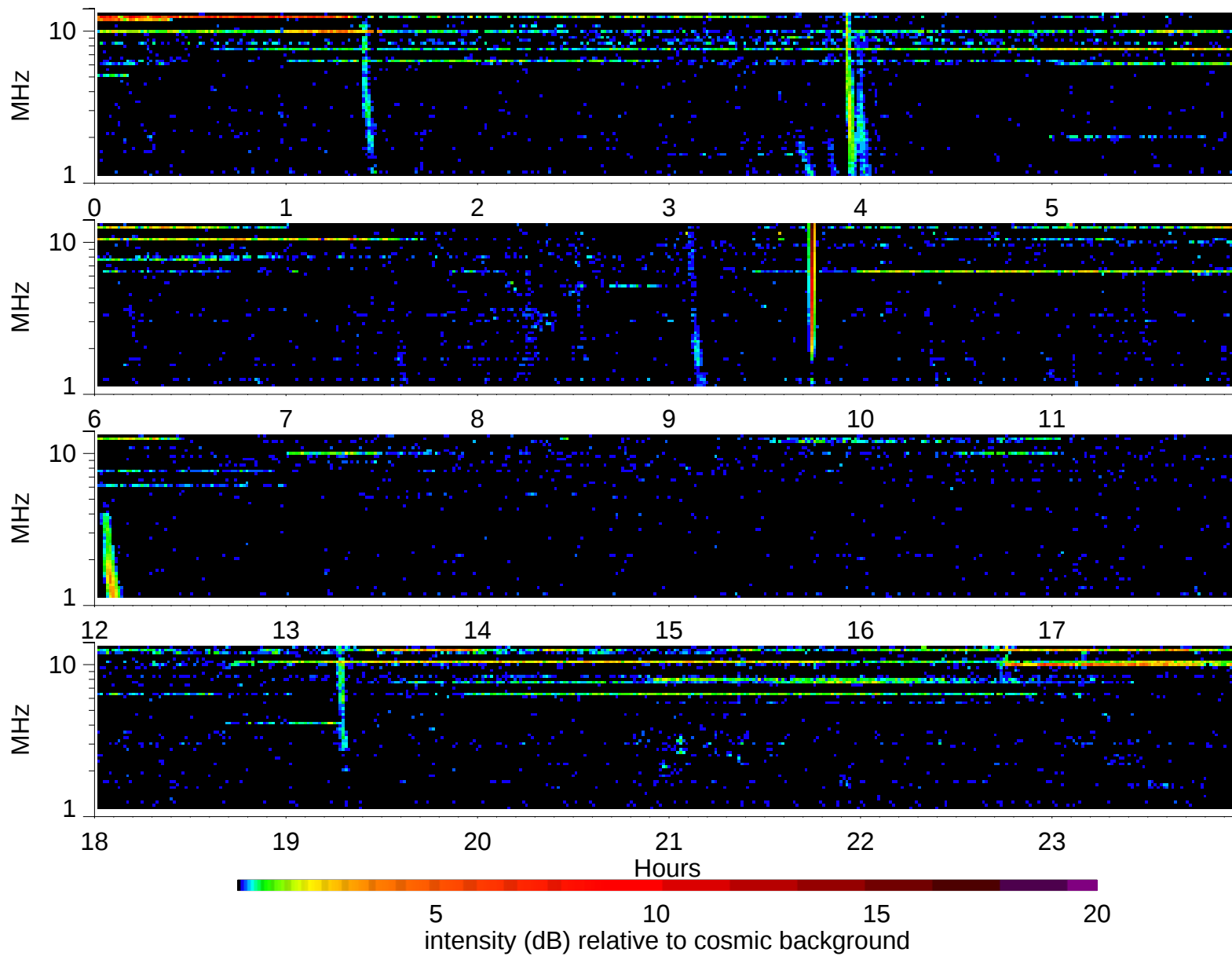
Wind Waves RAD2 receiver: 2002/1/17
