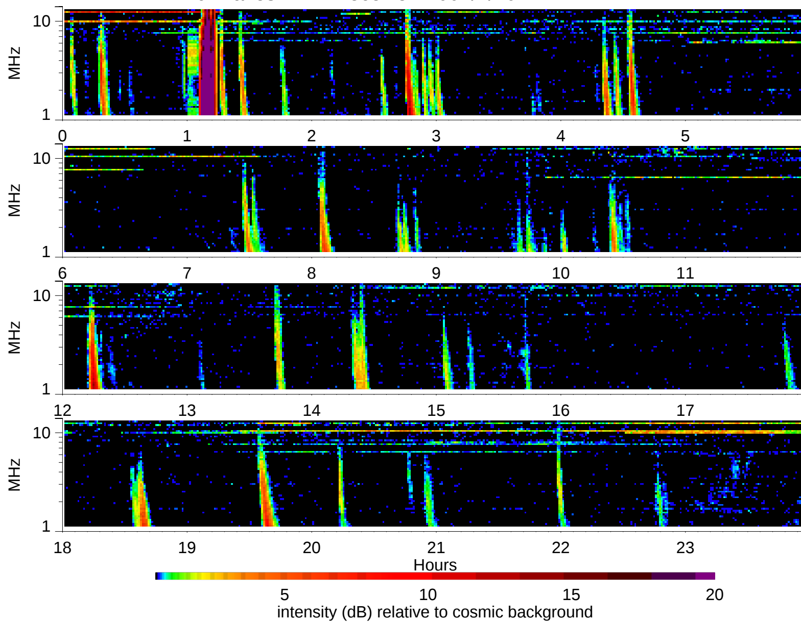
Wind Waves RAD2 receiver: 2002/1/20
