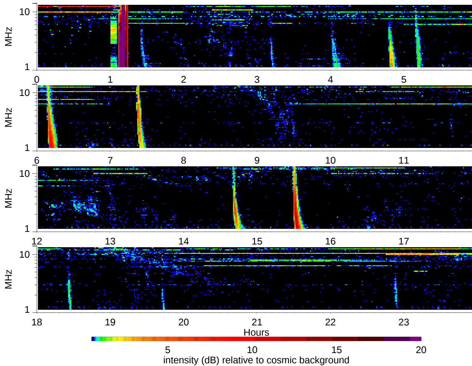
Wind Waves RAD2 receiver: 2002/1/24
