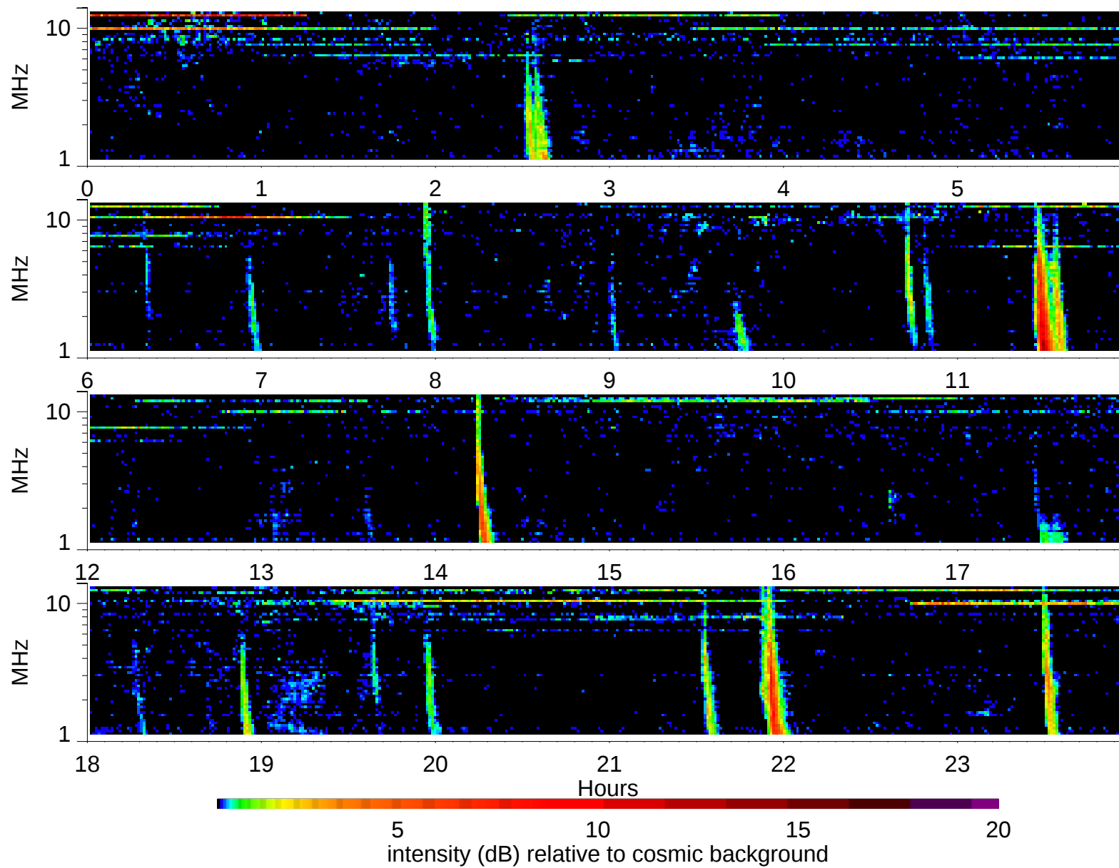
Wind Waves RAD2 receiver: 2002/1/25
