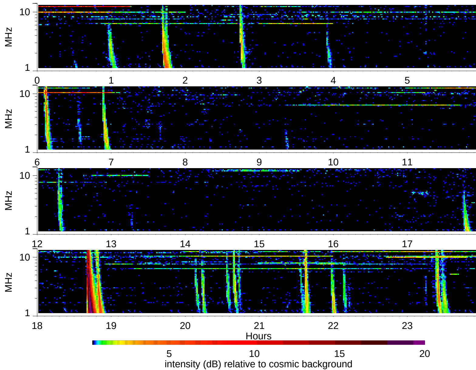
Wind Waves RAD2 receiver: 2002/1/29
