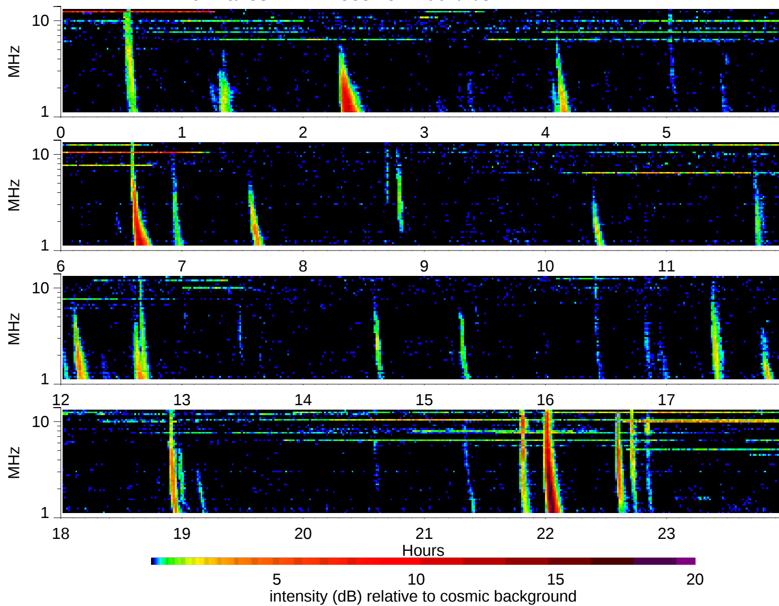
Wind Waves RAD2 receiver: 2002/1/31
