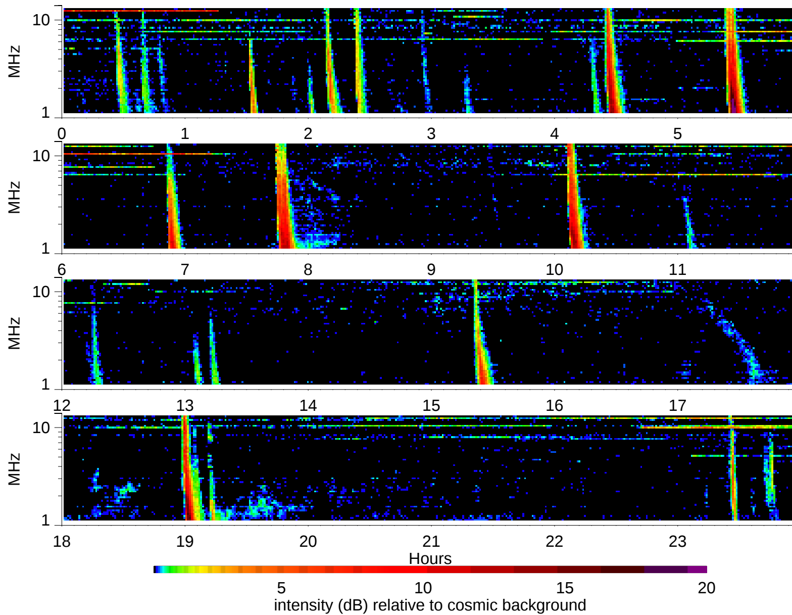
Wind Waves RAD2 receiver: 2002/2/4
