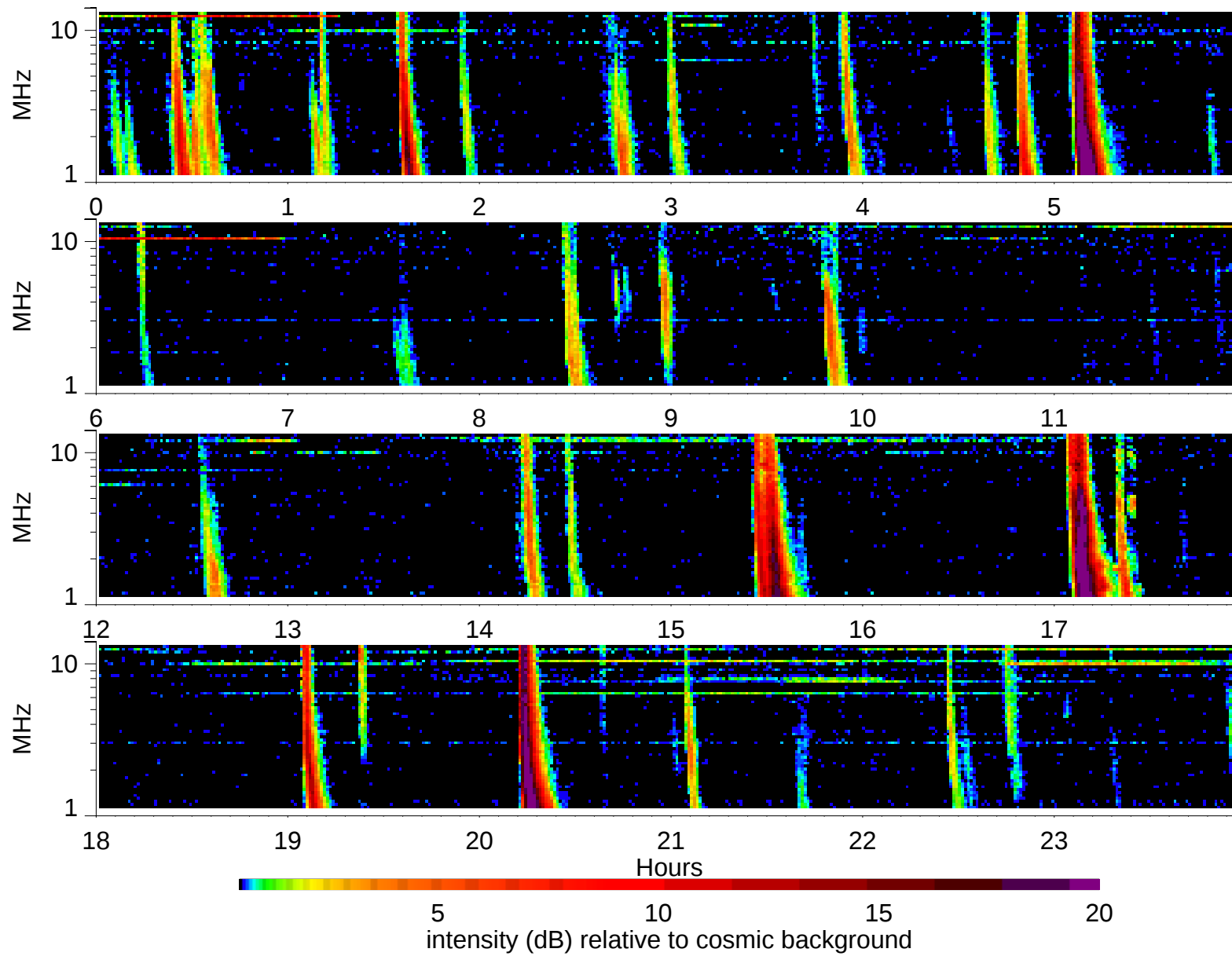
Wind Waves RAD2 receiver: 2002/2/6
