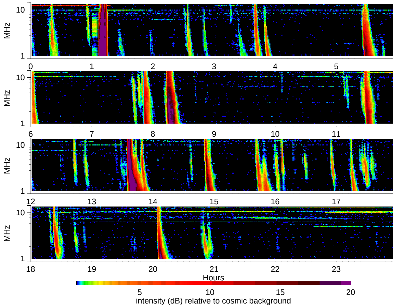
Wind Waves RAD2 receiver: 2002/2/7
