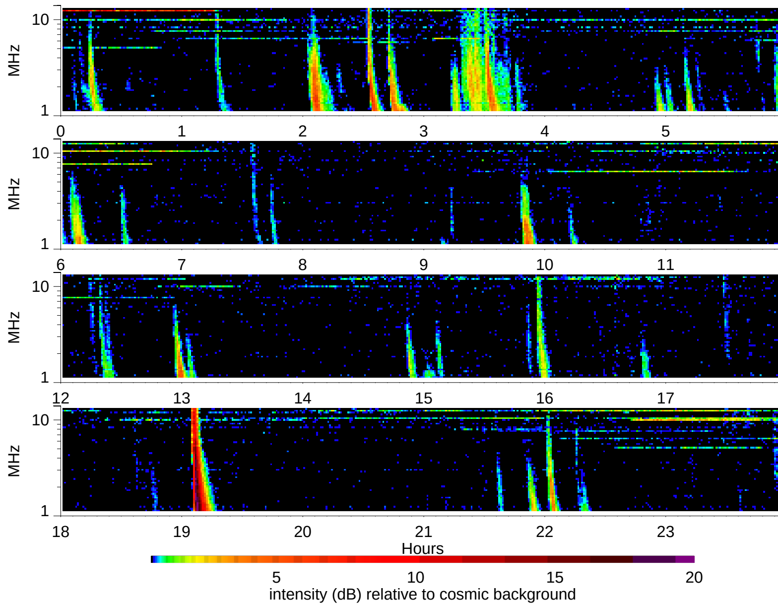
Wind Waves RAD2 receiver: 2002/2/8
