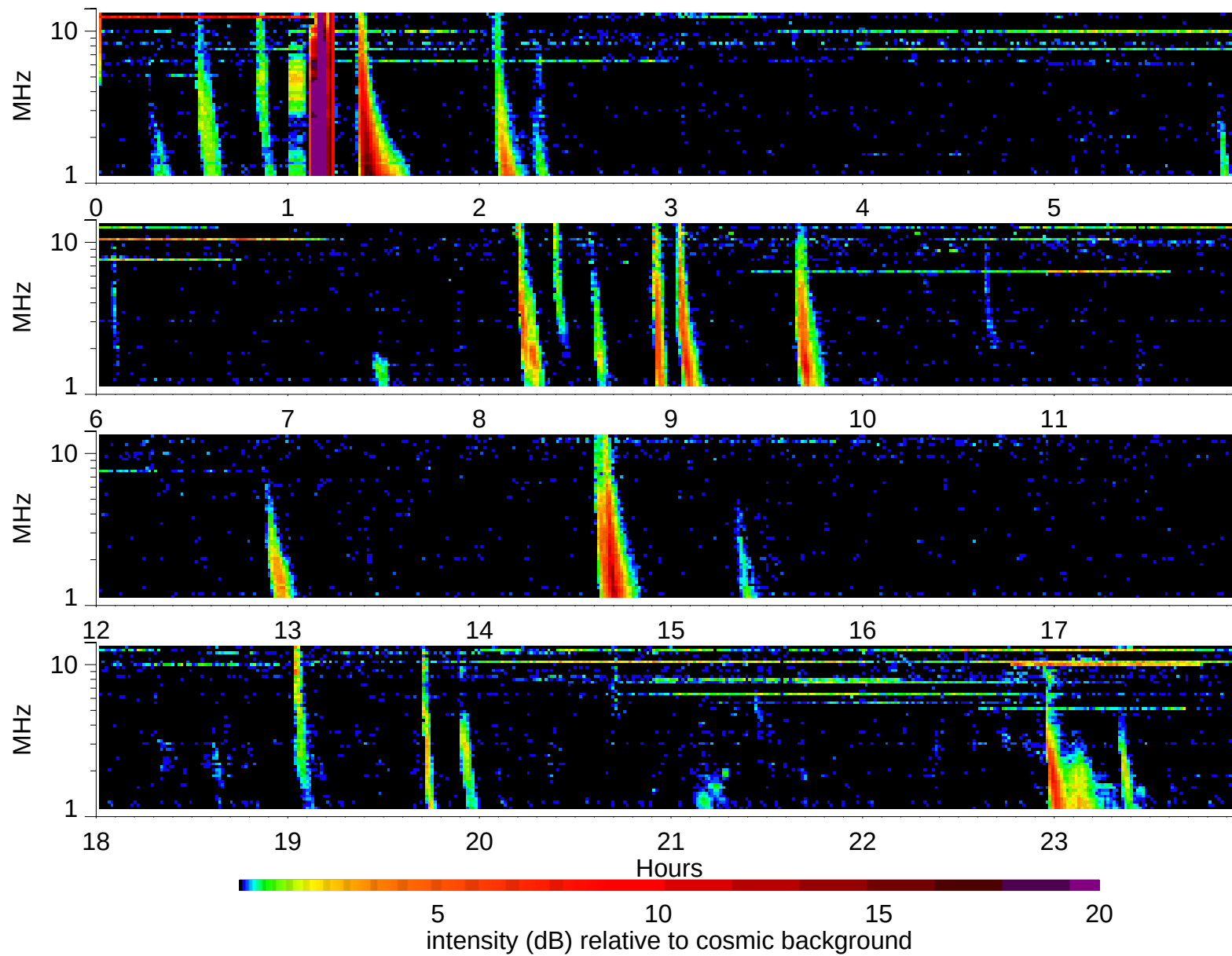
Wind Waves RAD2 receiver: 2002/2/9
