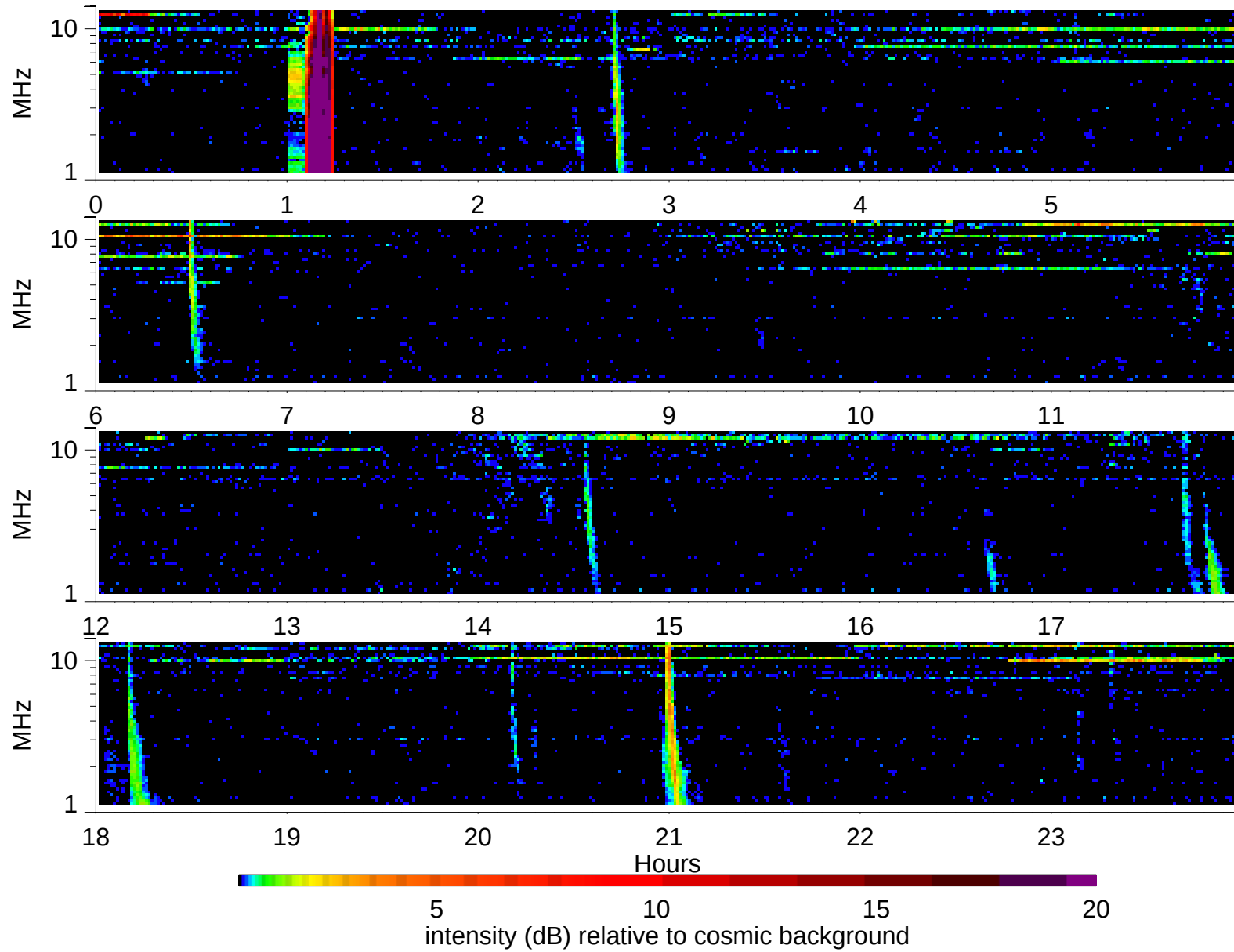
Wind Waves RAD2 receiver: 2002/2/11
