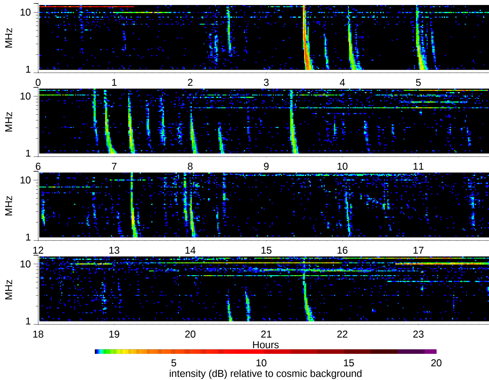
Wind Waves RAD2 receiver: 2002/2/12
