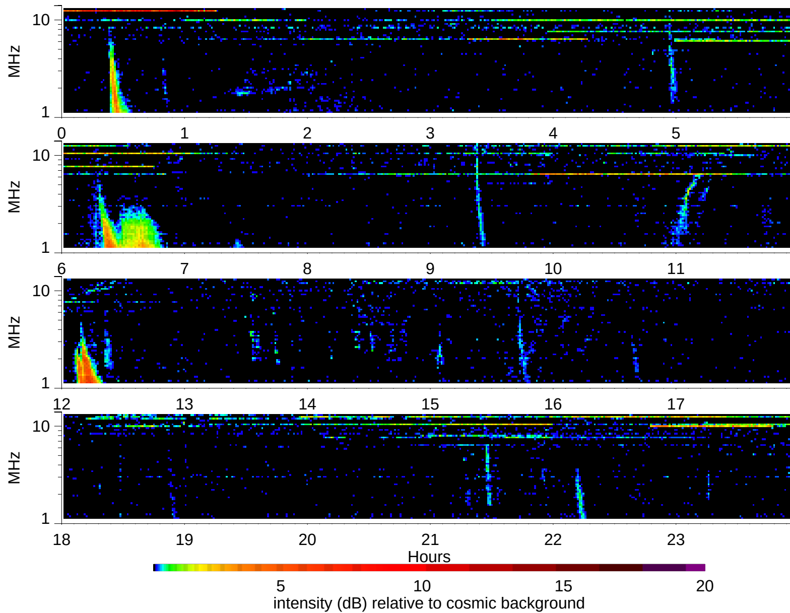
Wind Waves RAD2 receiver: 2002/2/16
