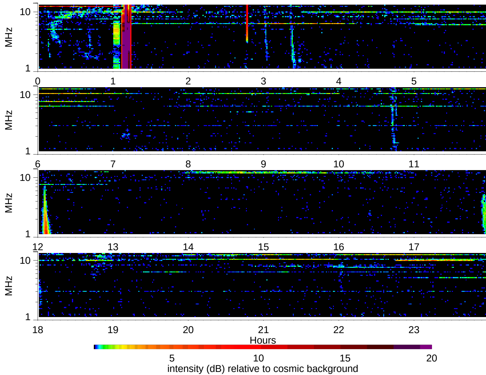
Wind Waves RAD2 receiver: 2002/2/17
