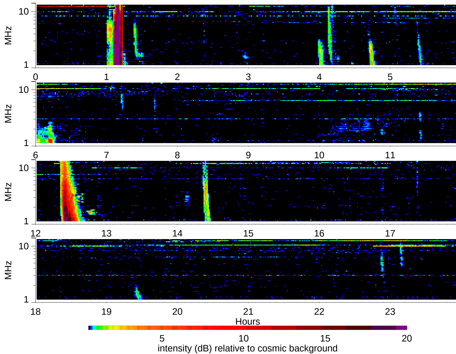
Wind Waves RAD2 receiver: 2002/2/21
