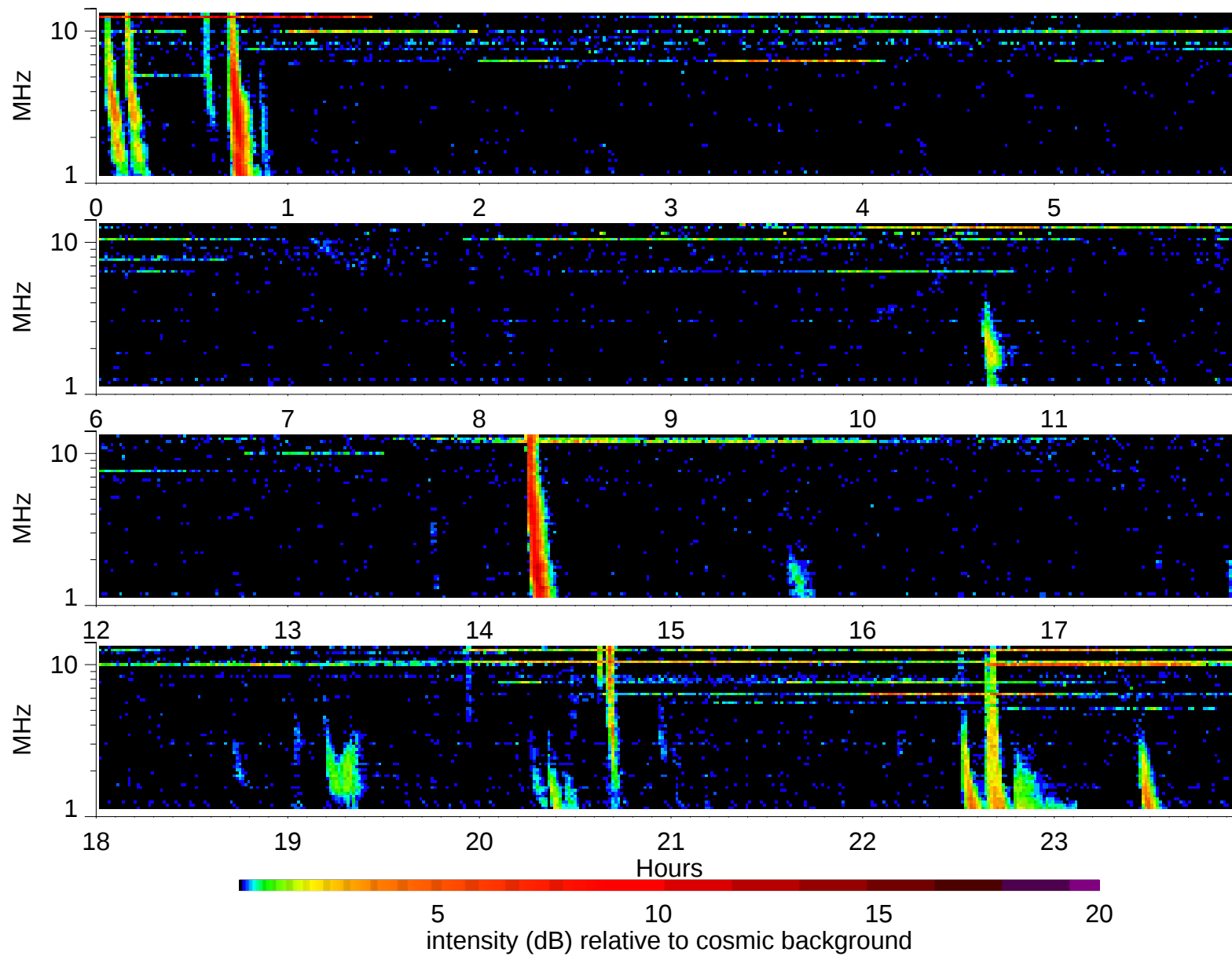
Wind Waves RAD2 receiver: 2002/2/28
