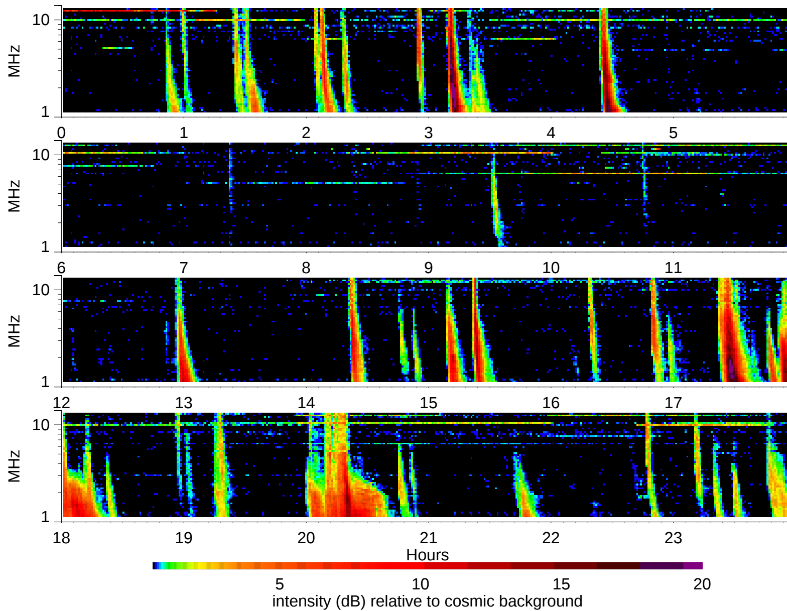
Wind Waves RAD2 receiver: 2002/3/2
