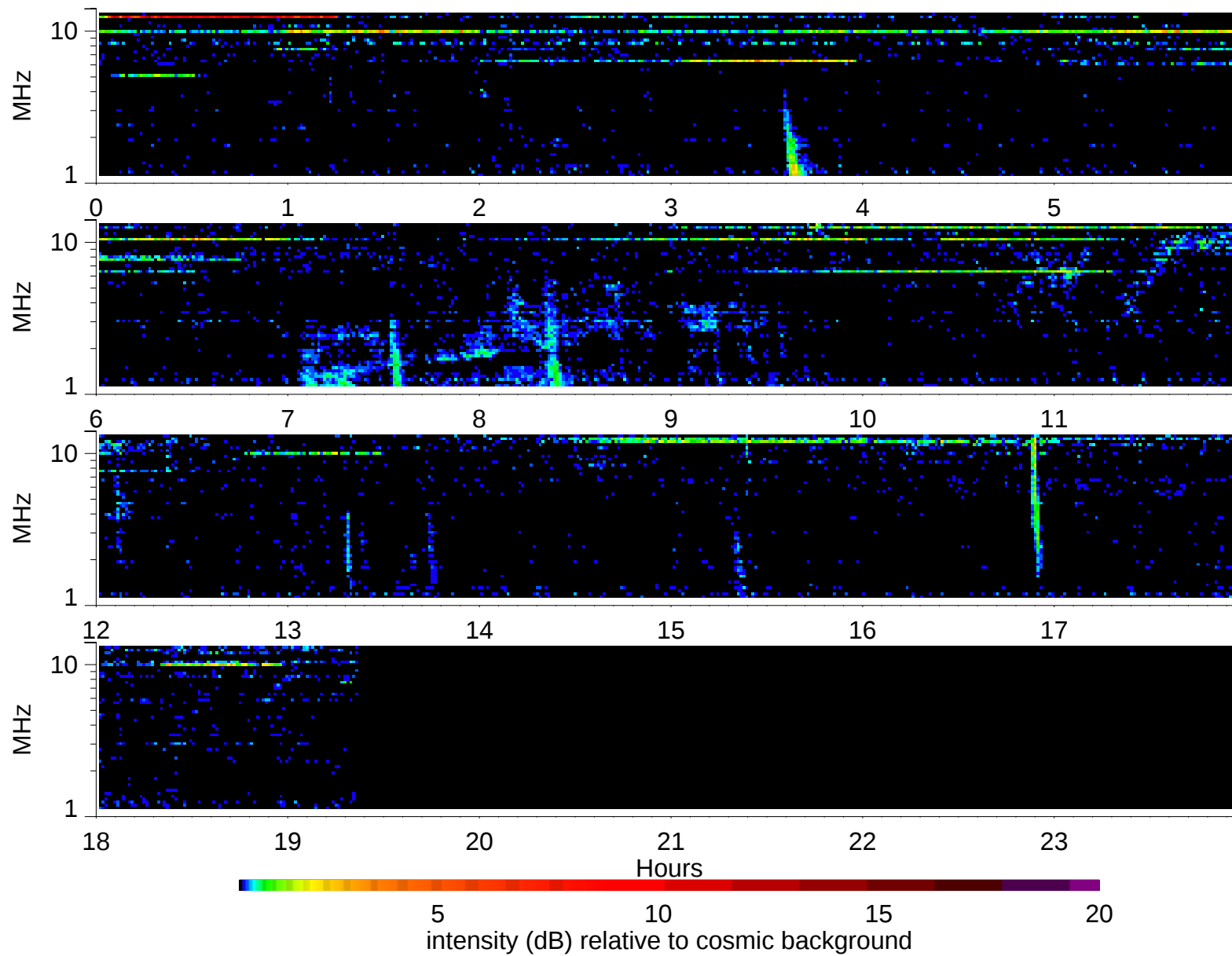
Wind Waves RAD2 receiver: 2002/3/8
