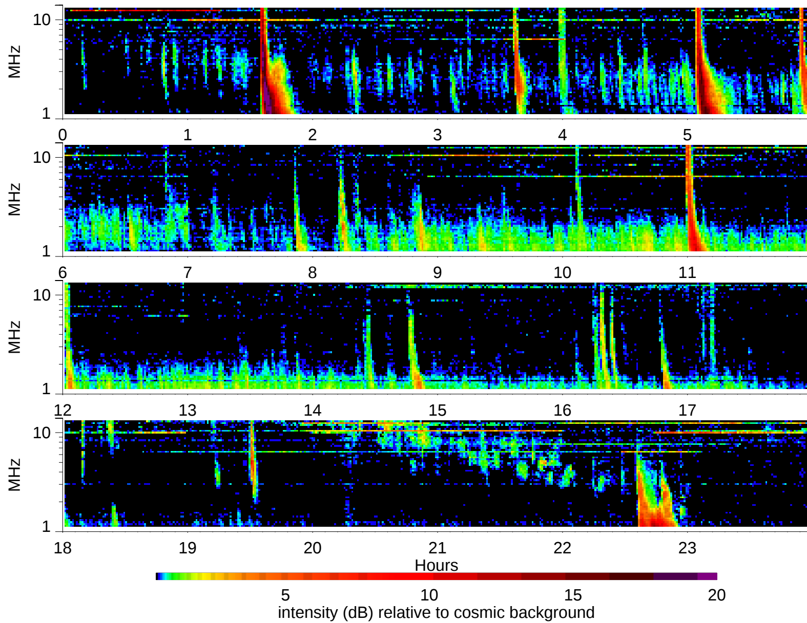
Wind Waves RAD2 receiver: 2002/3/10
