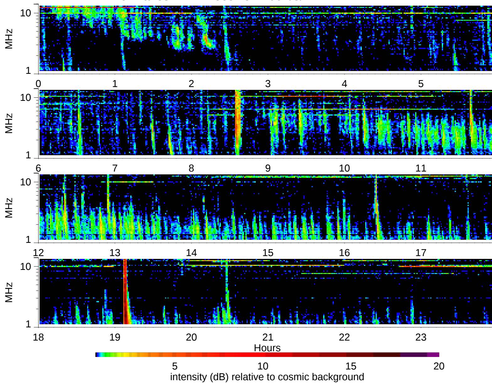
Wind Waves RAD2 receiver: 2002/3/12
