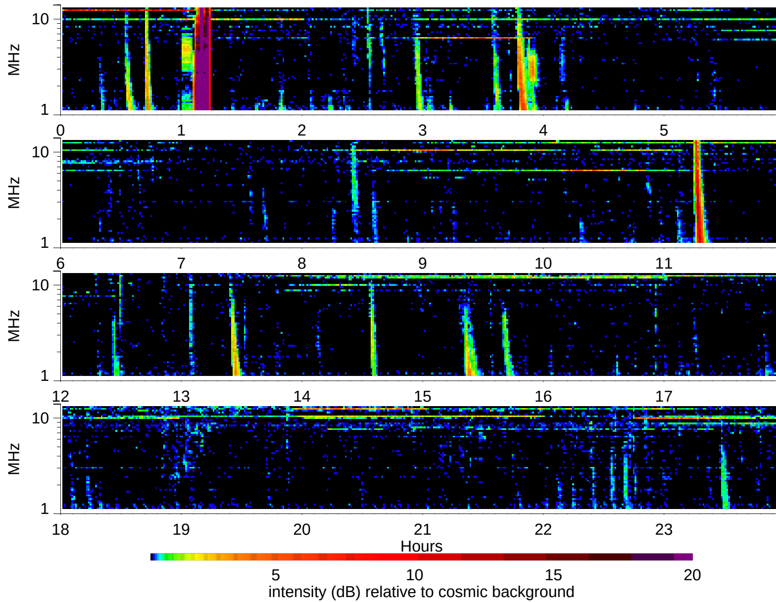
Wind Waves RAD2 receiver: 2002/3/13
