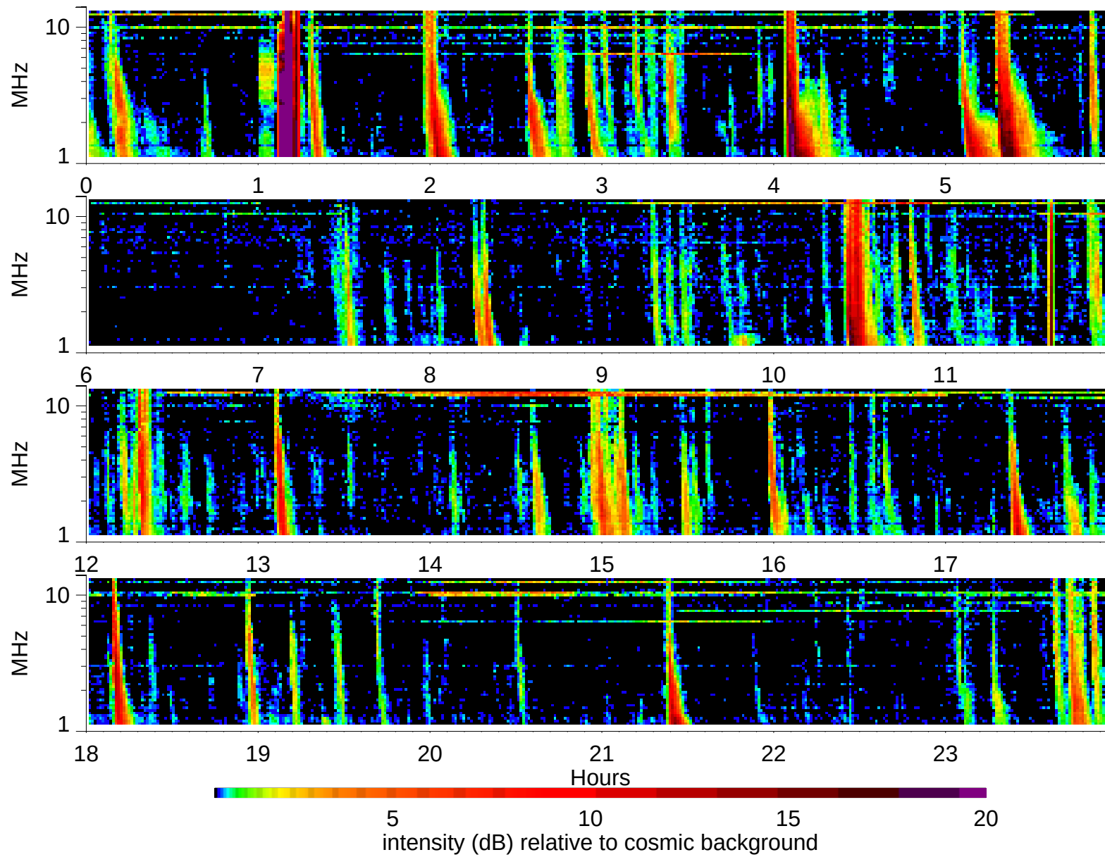
Wind Waves RAD2 receiver: 2002/3/19
