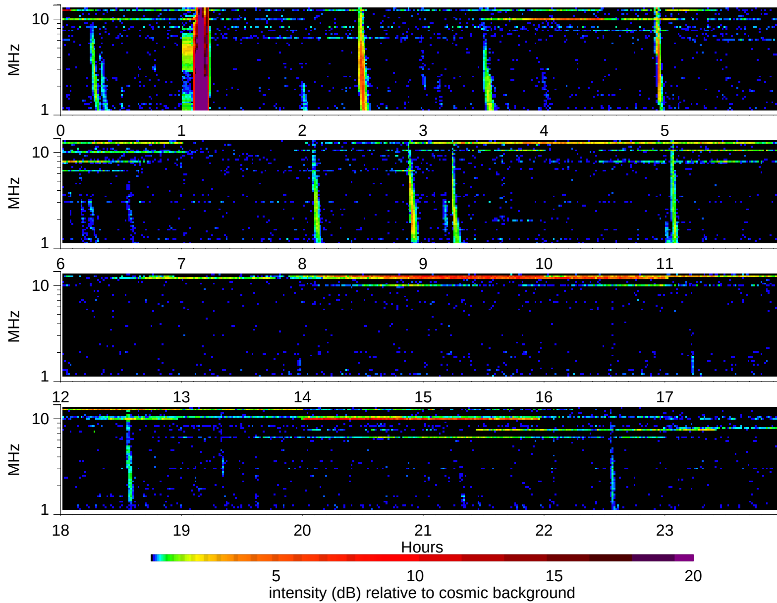
Wind Waves RAD2 receiver: 2002/3/23
