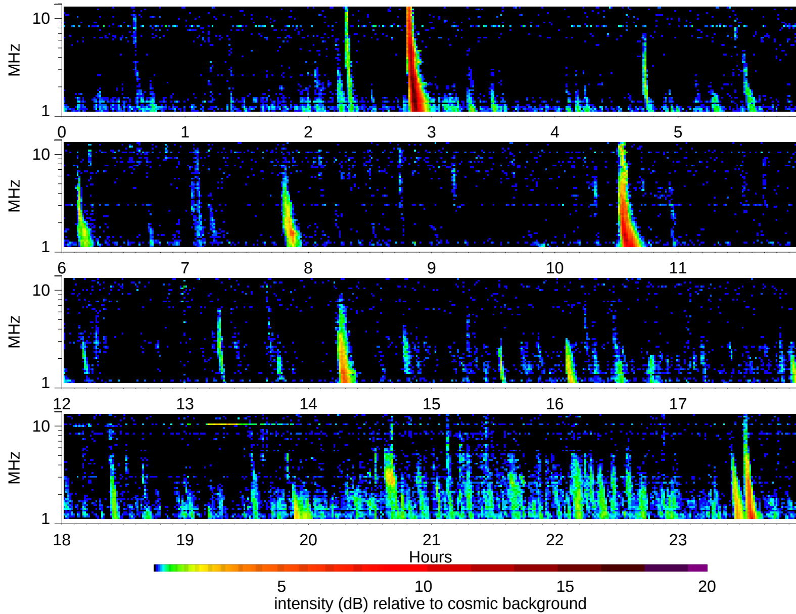
Wind Waves RAD2 receiver: 2002/3/30
