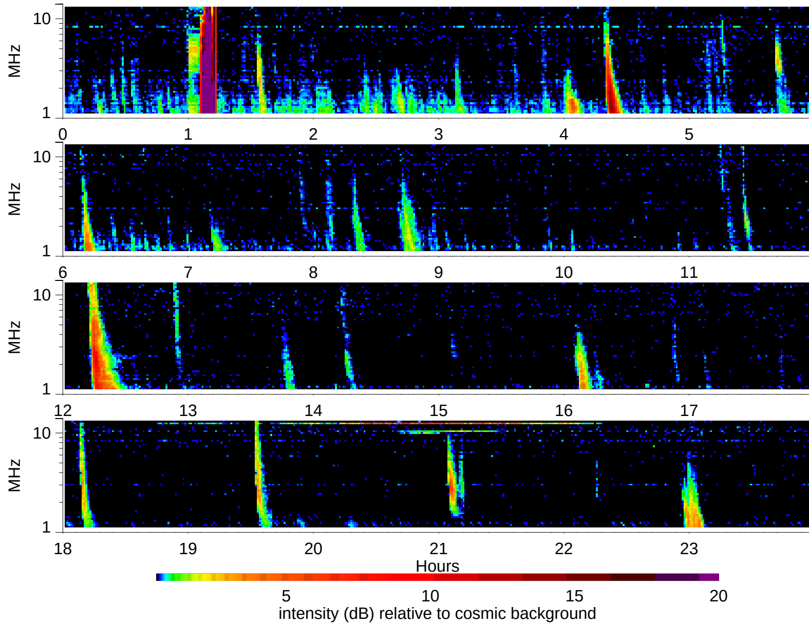
Wind Waves RAD2 receiver: 2002/3/31
