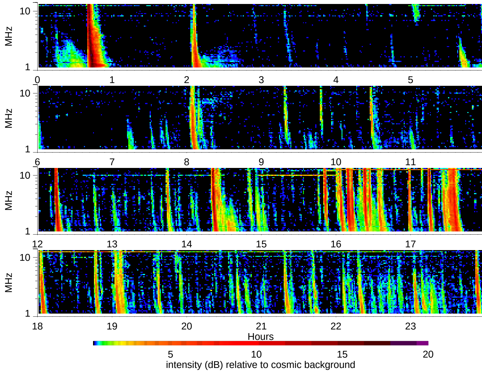
Wind Waves RAD2 receiver: 2002/4/9
