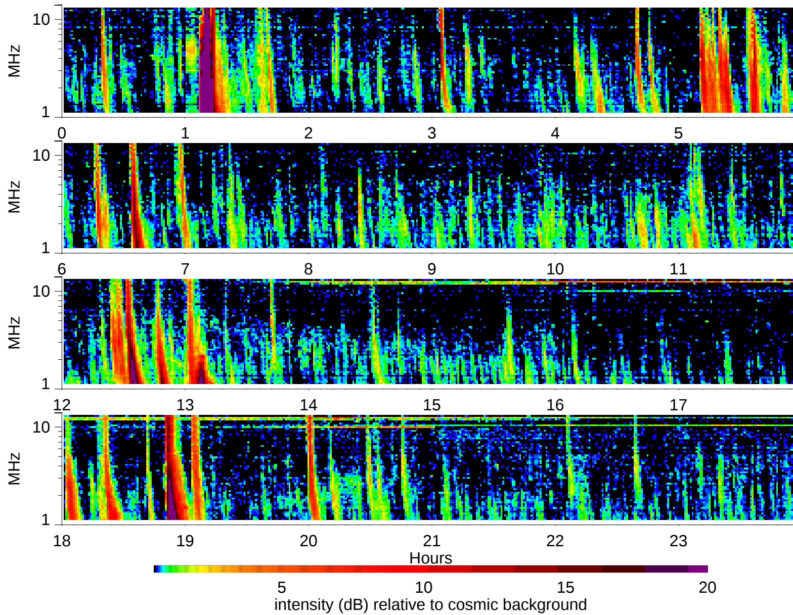
Wind Waves RAD2 receiver: 2002/4/10
