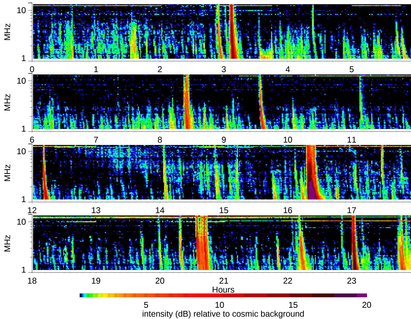
Wind Waves RAD2 receiver: 2002/4/11
