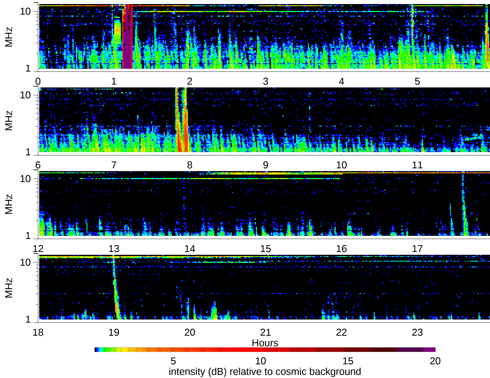
Wind Waves RAD2 receiver: 2002/4/12
