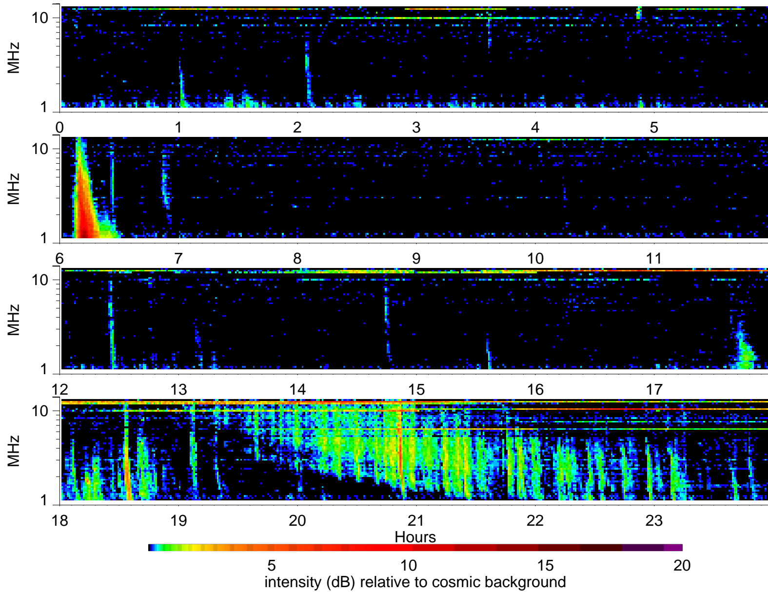
Wind Waves RAD2 receiver: 2002/4/13
