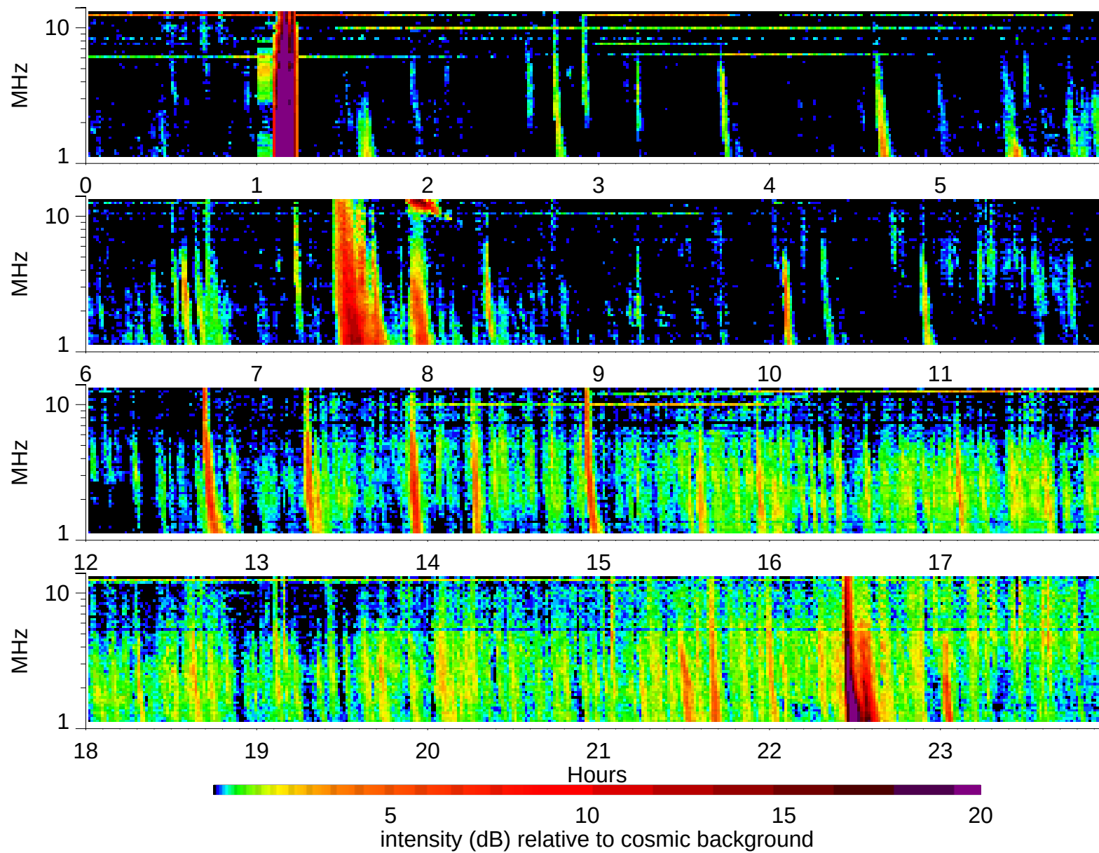
Wind Waves RAD2 receiver: 2002/4/14
