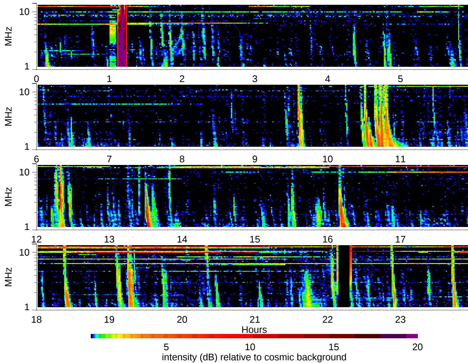
Wind Waves RAD2 receiver: 2002/4/18
