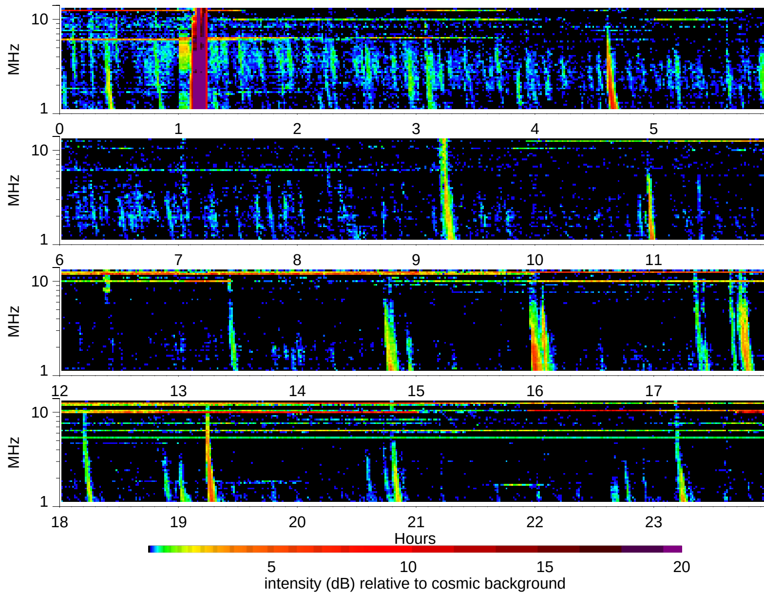
Wind Waves RAD2 receiver: 2002/4/20
