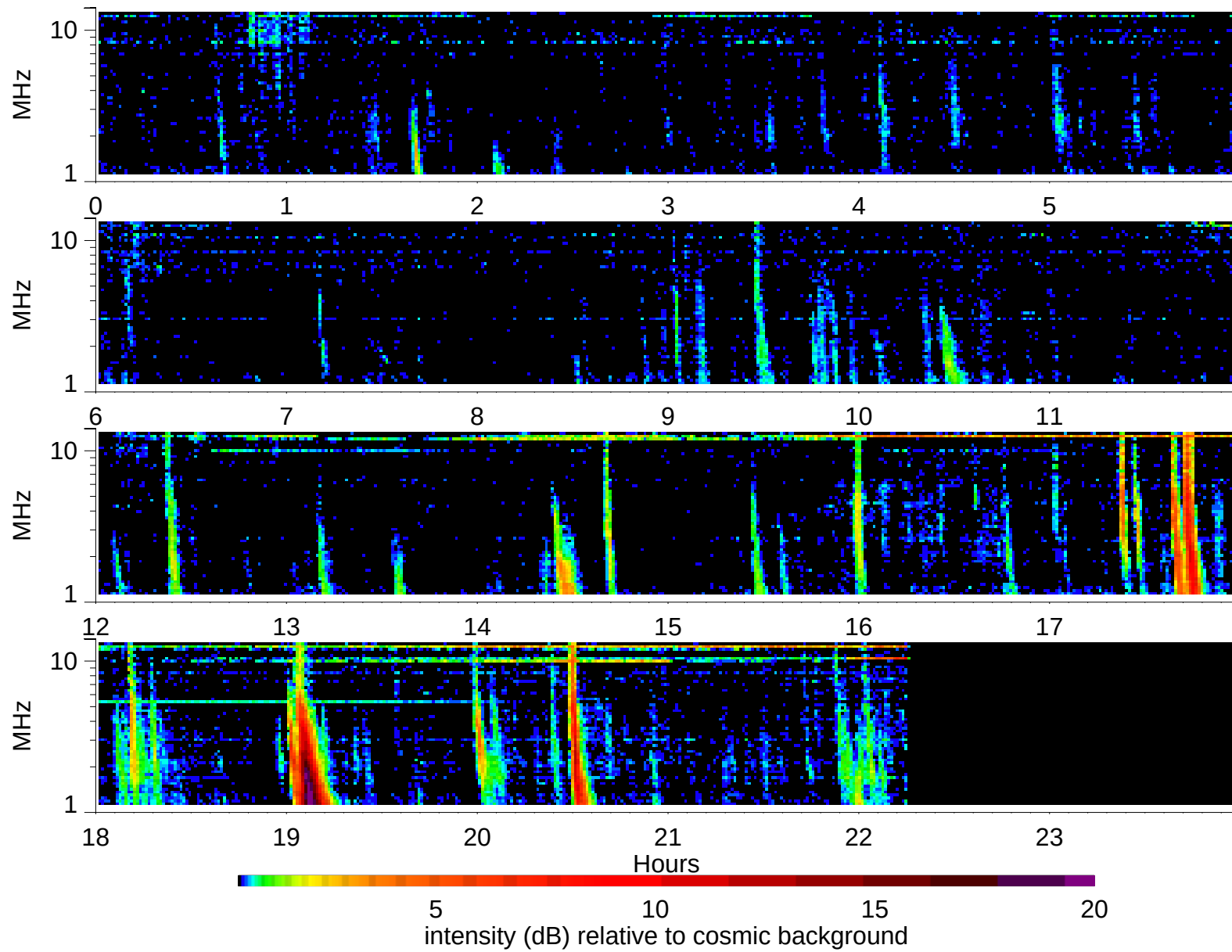
Wind Waves RAD2 receiver: 2002/4/23
