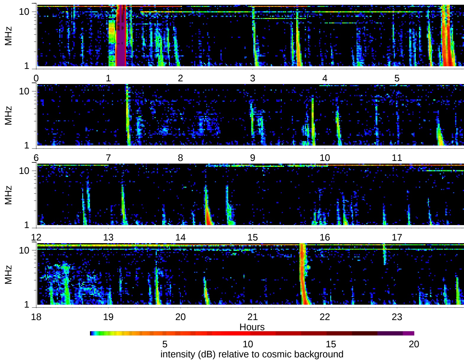
Wind Waves RAD2 receiver: 2002/4/28
