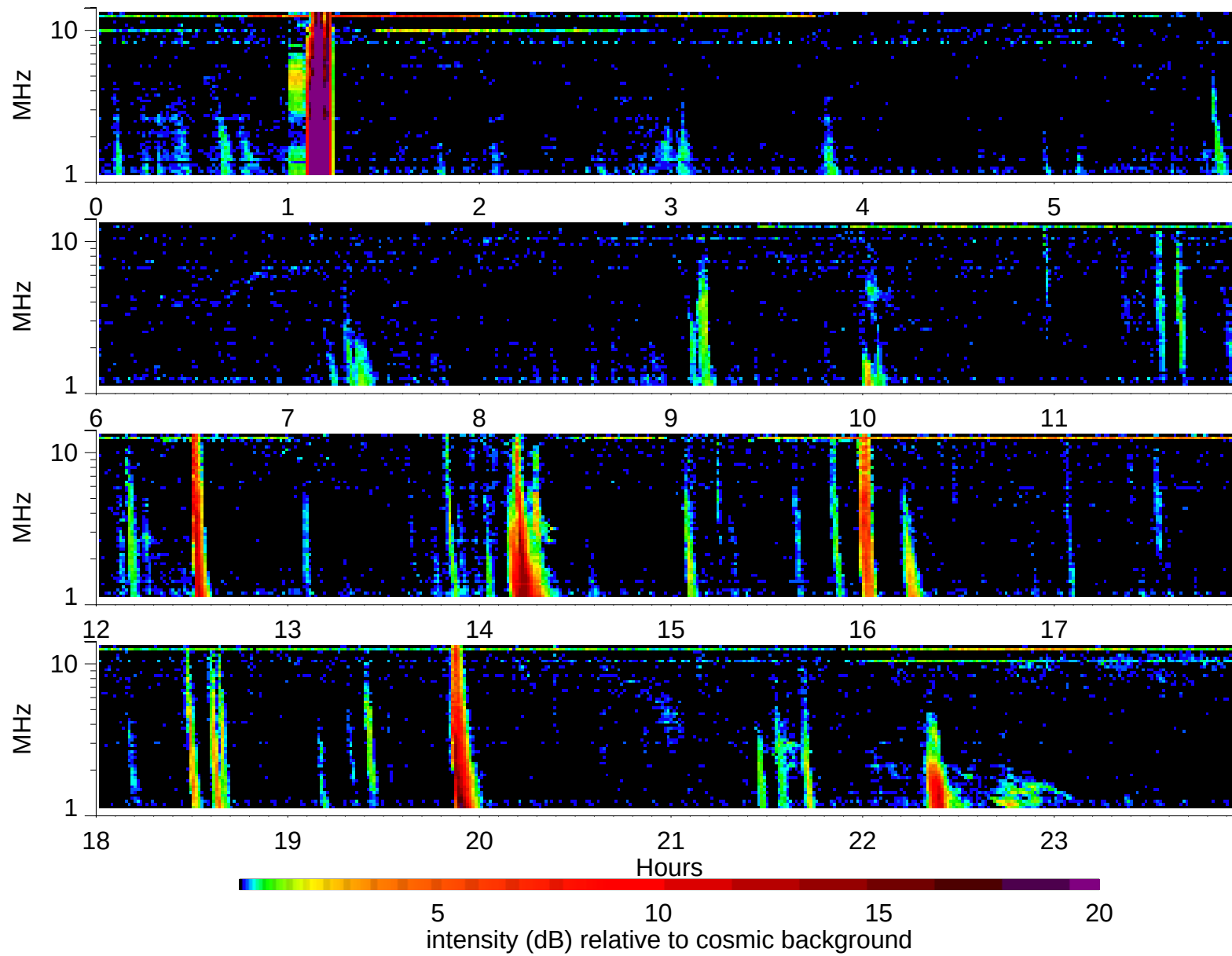
Wind Waves RAD2 receiver: 2002/4/30
