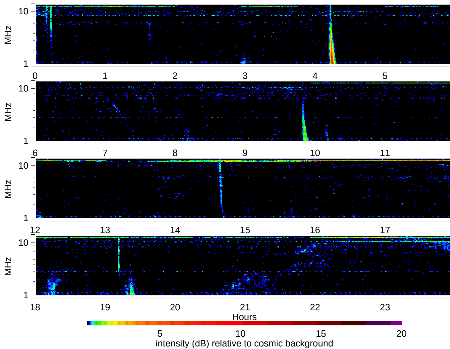
Wind Waves RAD2 receiver: 2002/5/1
