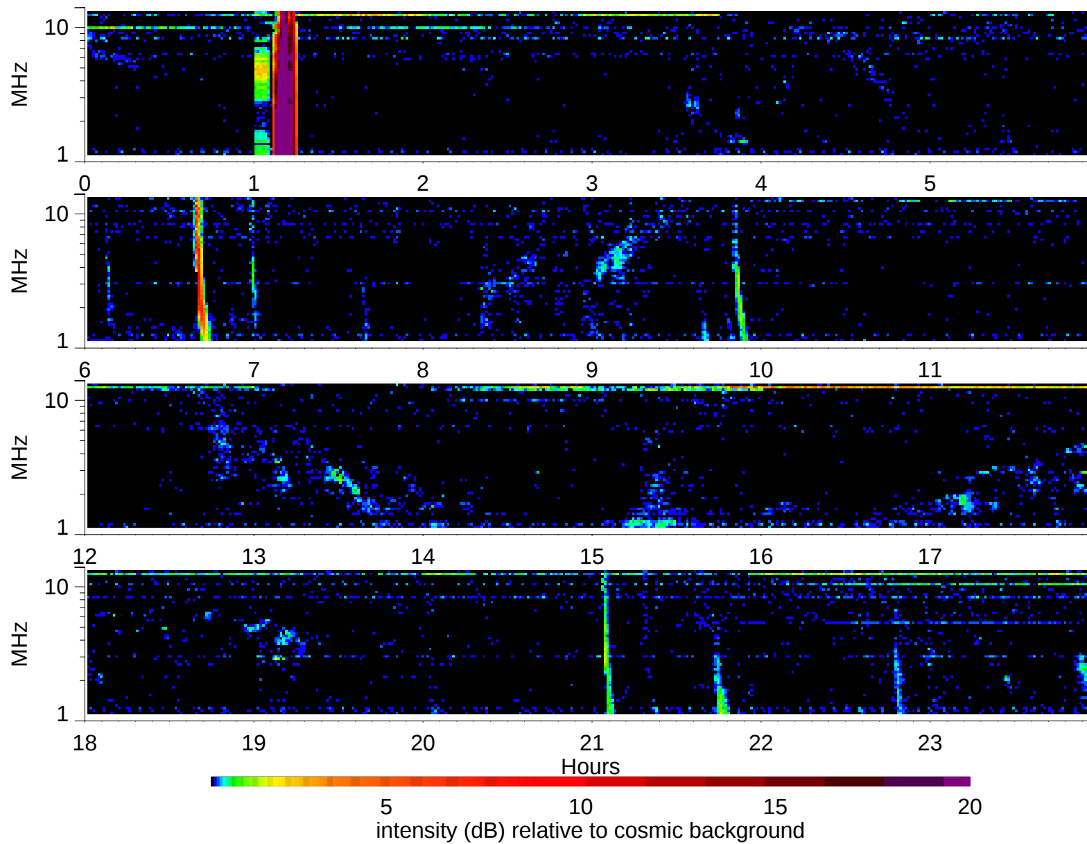
Wind Waves RAD2 receiver: 2002/5/2
