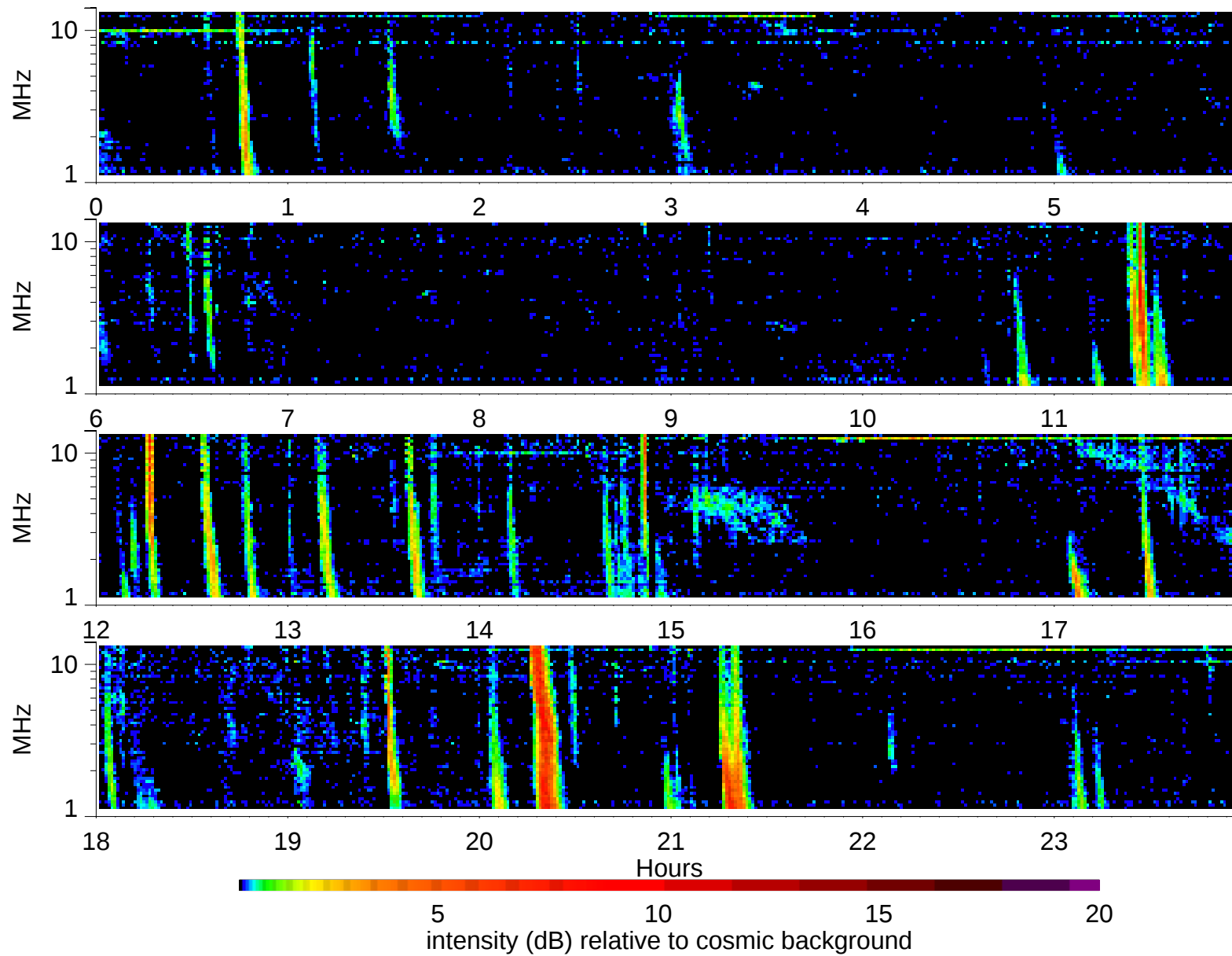
Wind Waves RAD2 receiver: 2002/5/3
