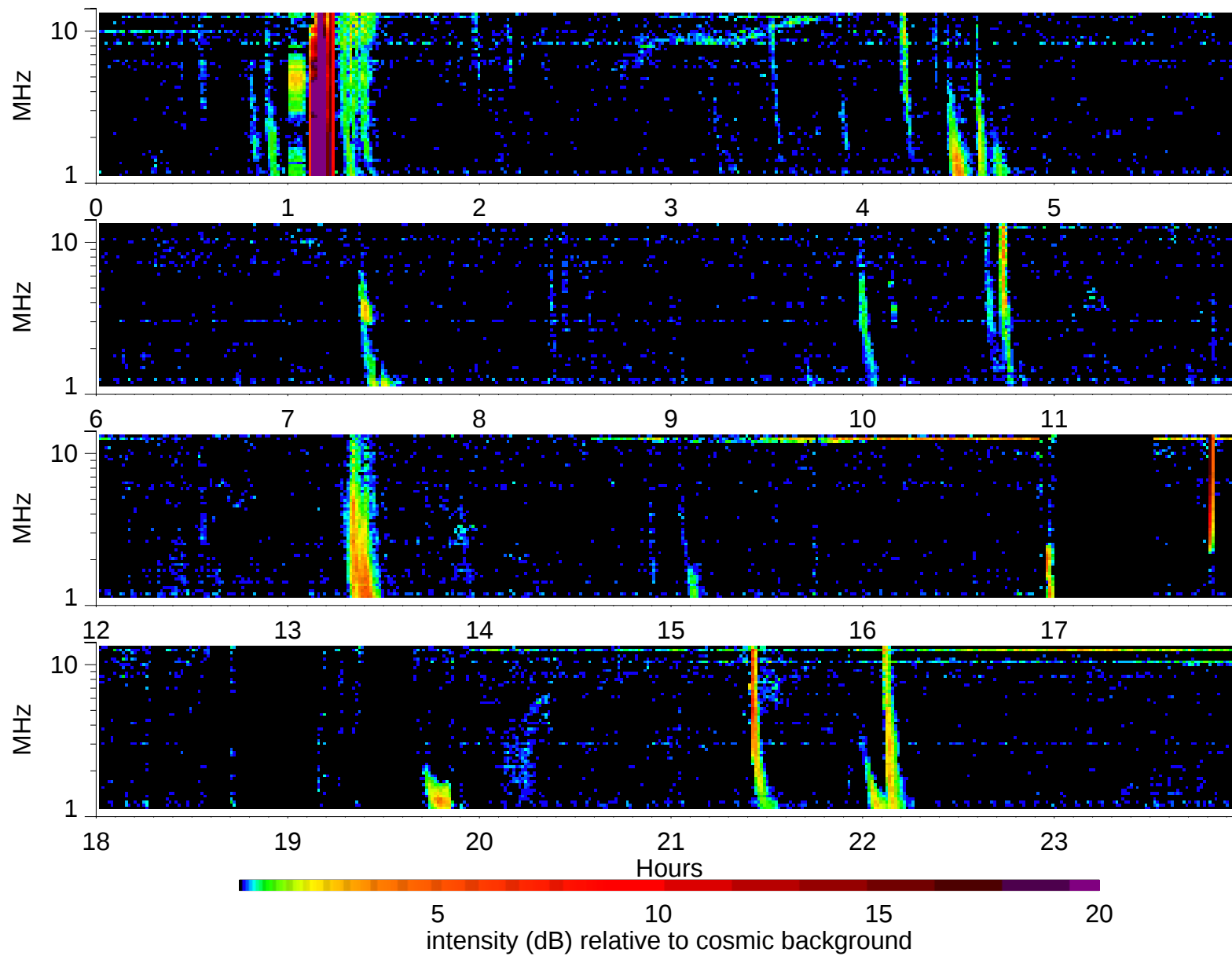
Wind Waves RAD2 receiver: 2002/5/4
