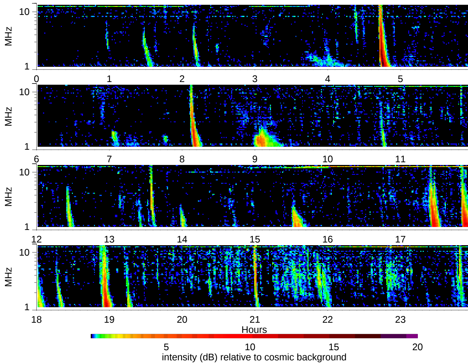
Wind Waves RAD2 receiver: 2002/5/5
