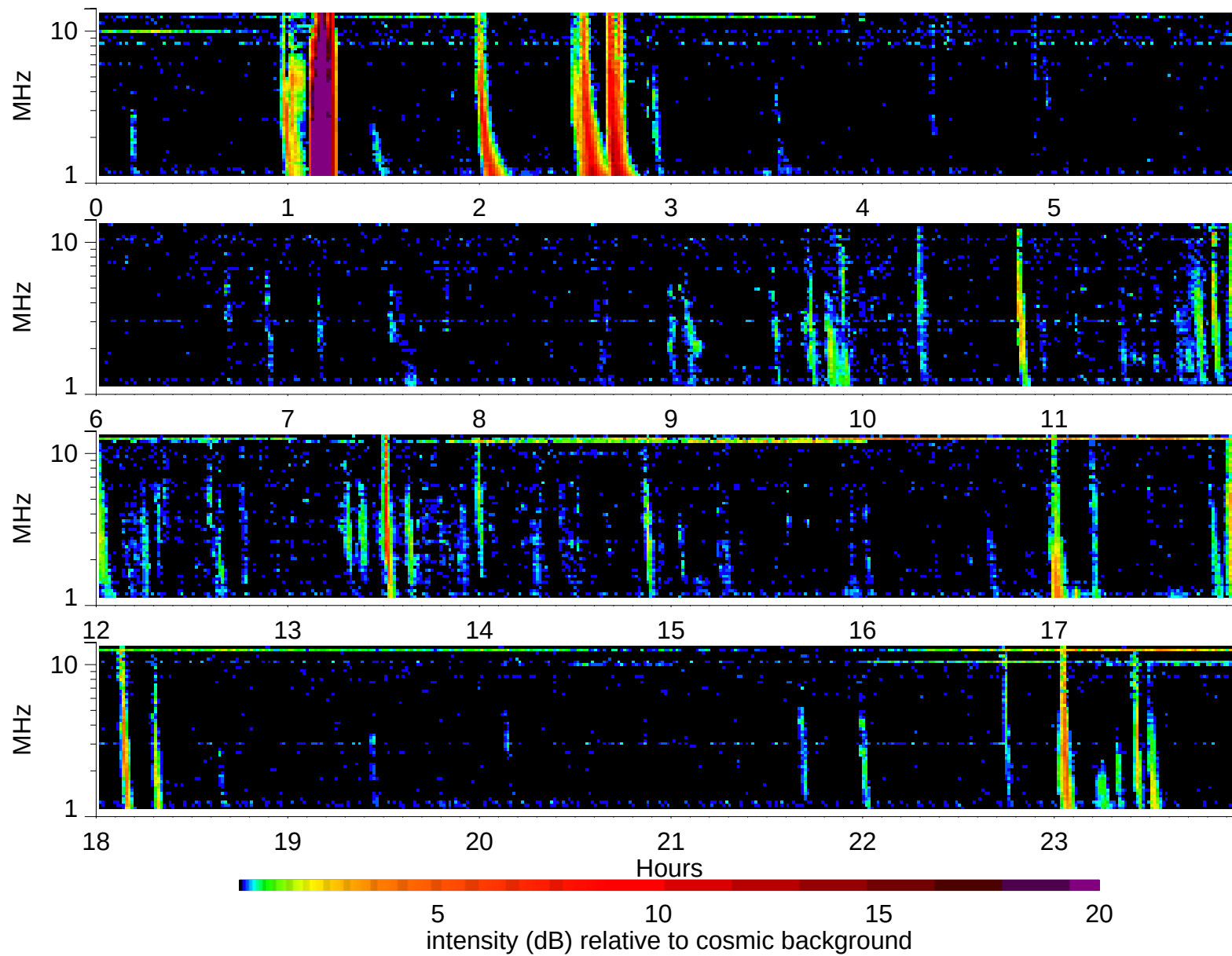
Wind Waves RAD2 receiver: 2002/5/10
